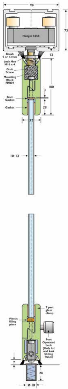
Multidirectional door
